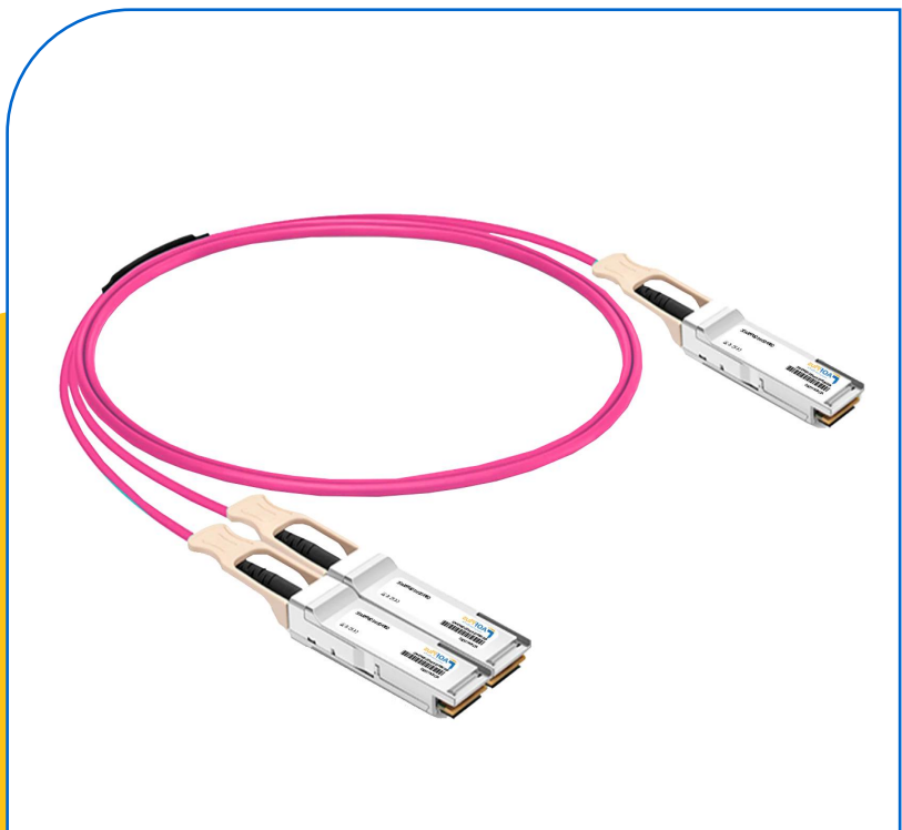
400G OSFP to 2x200G QSFP56 OM4 Active Optical Breakout Cable
